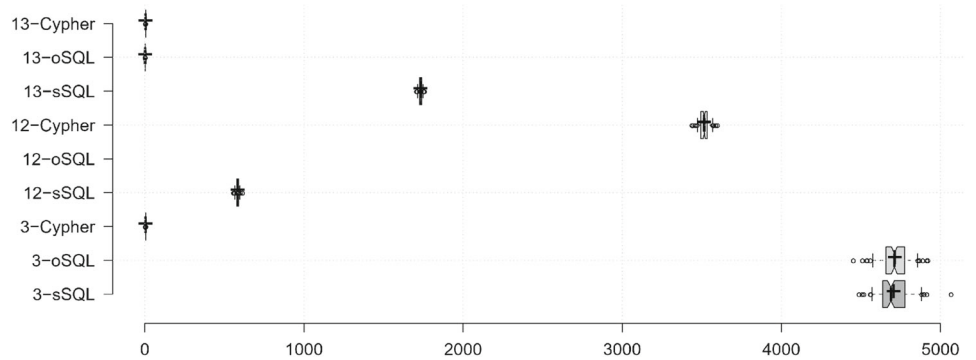
Fig. 11 Queries with high execution time in ms, overview of all formulation times
