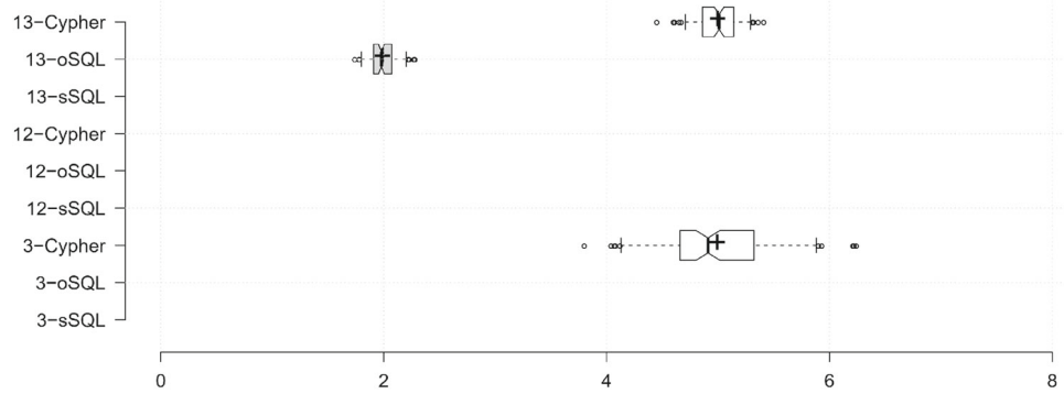
Fig. 12 Queries with high execution time in ms, zoom on formulations with low execution time
