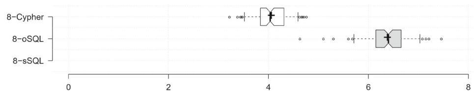
Fig. 14 Queries with very high execution time in ms, zoom on formulations with low execution time
