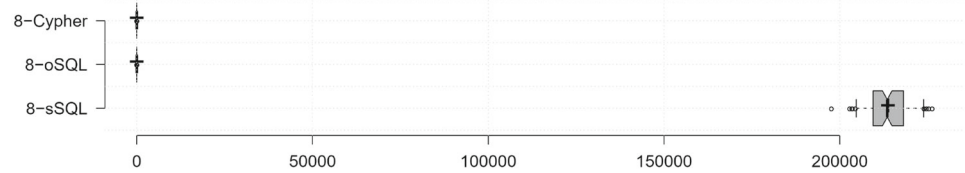
Fig. 13 Queries with very high execution time in ms, overview of all formulation times
