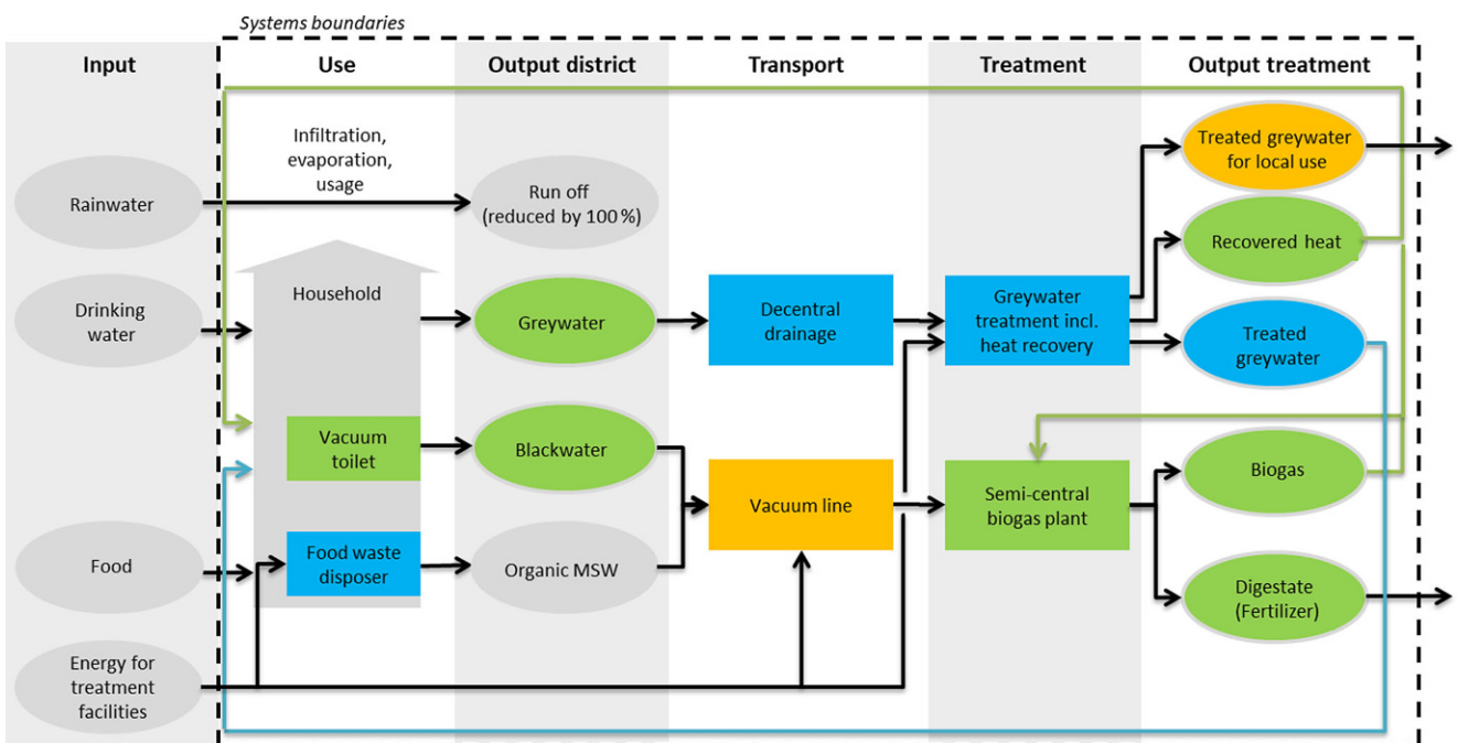
Fig. 4 System Alternative 3; the changes against the status quo are marked in orange, blue and green (Source: Friedrich et al. (2020))
