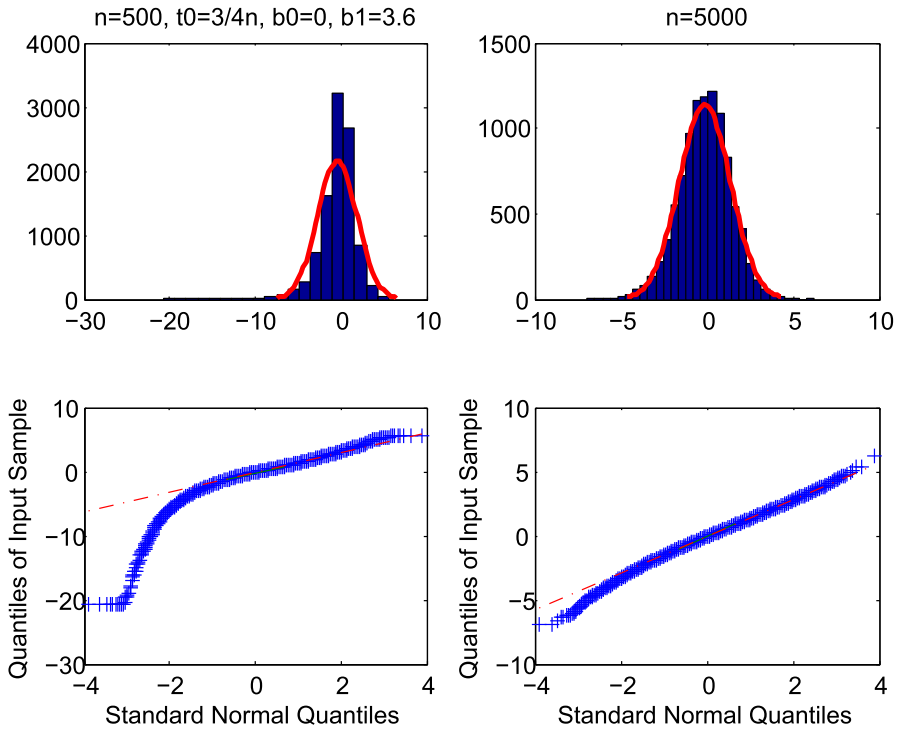
Fig. 3 Histograms and Q-Q plots of \sqrt{n}(\widehat{\tau}_0 - \tau_0) , left: n = 500 , right: n = 5000 , t_0 = 3n/4 , \beta_0 = 0 , \beta_1 = 3.6
