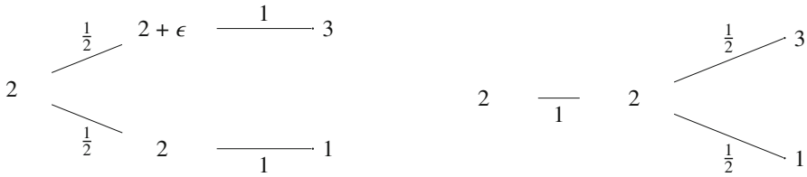
Fig. 1 Two processes illustrating two different flows of information, cf. Heitsch et al. (2006), Kovacevic and Pichler (2015). The arcs of the stochastic tree display the transition probabilities
