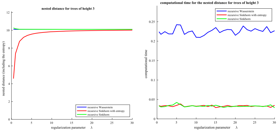
(a) Nested distance (blue) and Sinkhorn divergence (green, red) for regularization parameter \lambda \in \{0.5, 1, 2, \dots, 30\}
