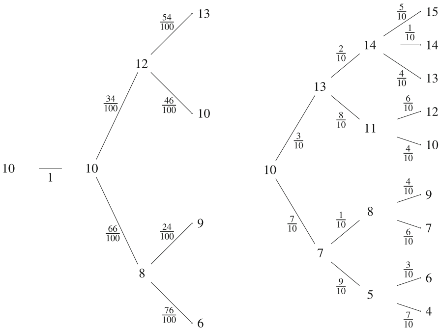
Fig. 3 Two arbitrary chosen processes with height T = 3
