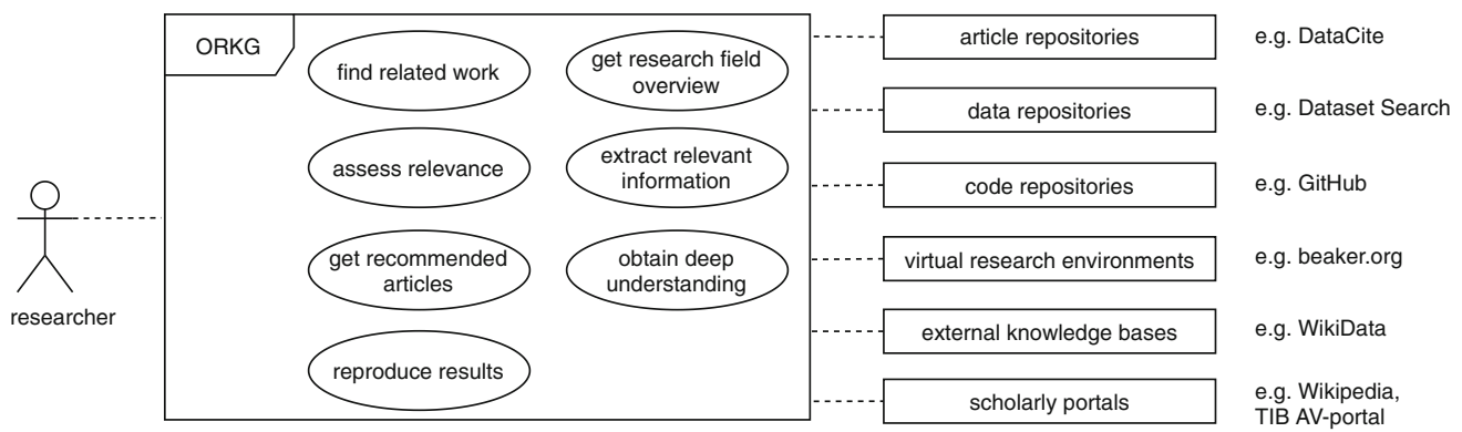
Fig. 2 UML use case diagram for the main use cases between a researcher, an Open Research Knowledge Graph (ORKG), and external systems
