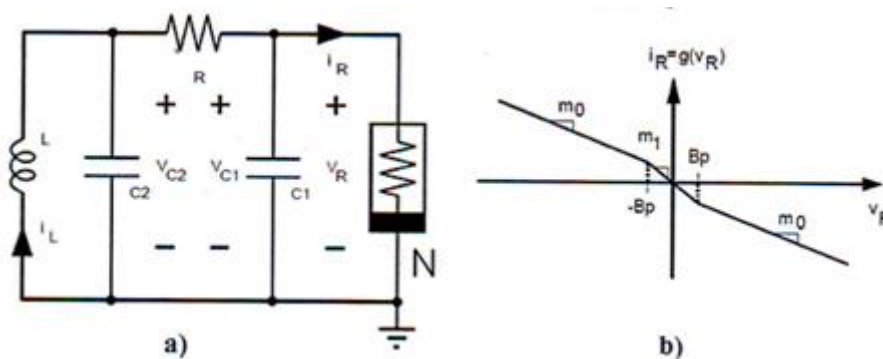
Figure 3. Basic diagram of the Chua simulator
