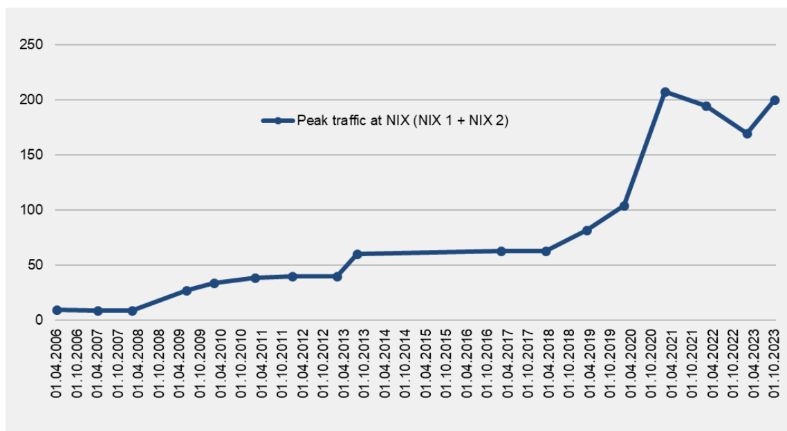
Figure 3-16: Peak Internet traffic at Oslo IXPs (NIX1 and 2) for 2006-2023 (Gbps)
