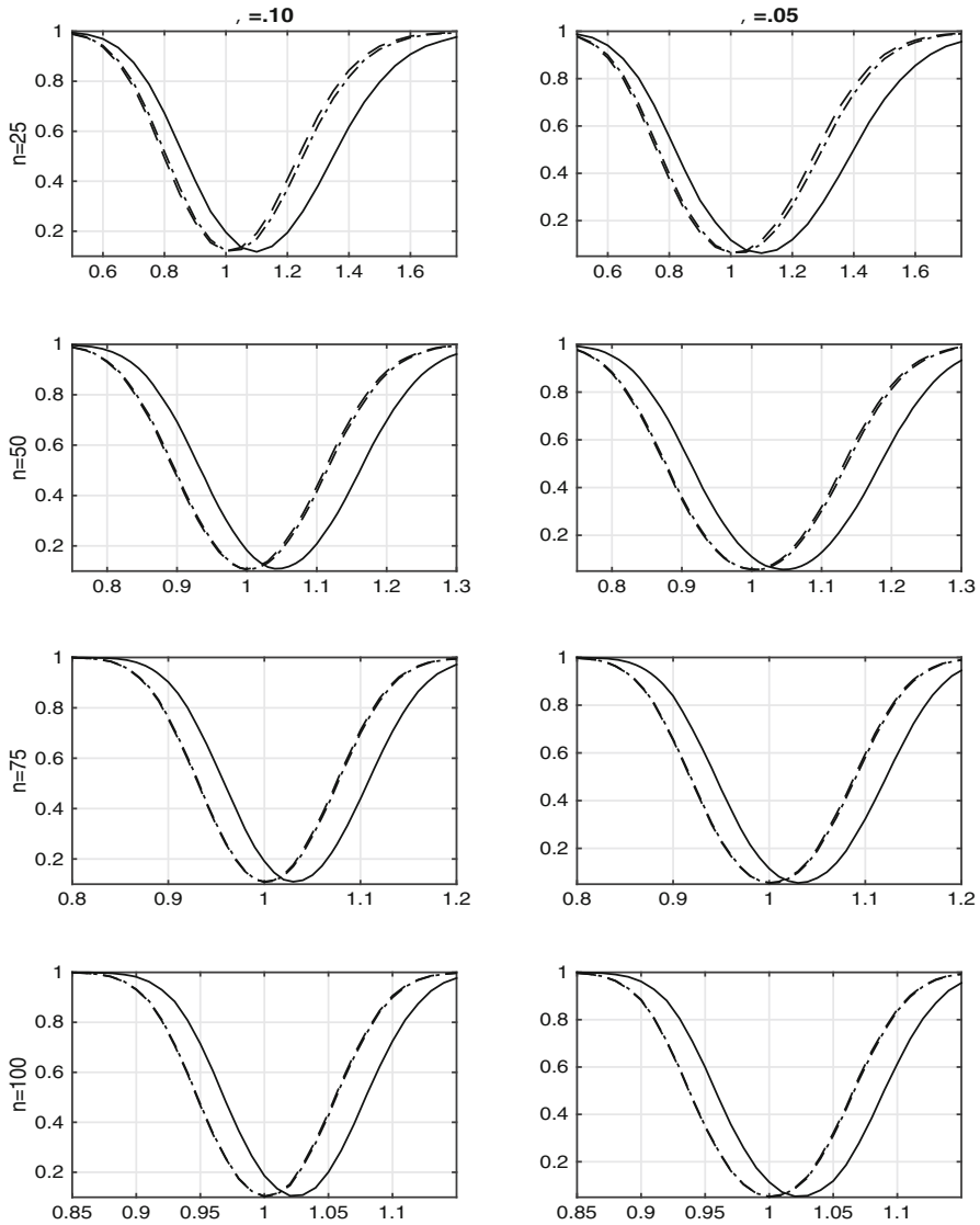
Fig. 1 Power curves. Design A1 for all n . Power curves for the likelihood ratio statistic based on the profile likelihood \hat{\ell}(\vartheta) (solid lines), the modified profile likelihood \check{\ell}(\vartheta) (dashed lines), and the modified profile likelihood that exploits the likelihood structure \check{\check{\ell}}(\vartheta) (dashed-dotted lines) for different sample sizes (vertically; n \in \{25, 50, 75, 100\} ) and size (horizontally; left: \alpha = .10 , right: \alpha = .05 )
