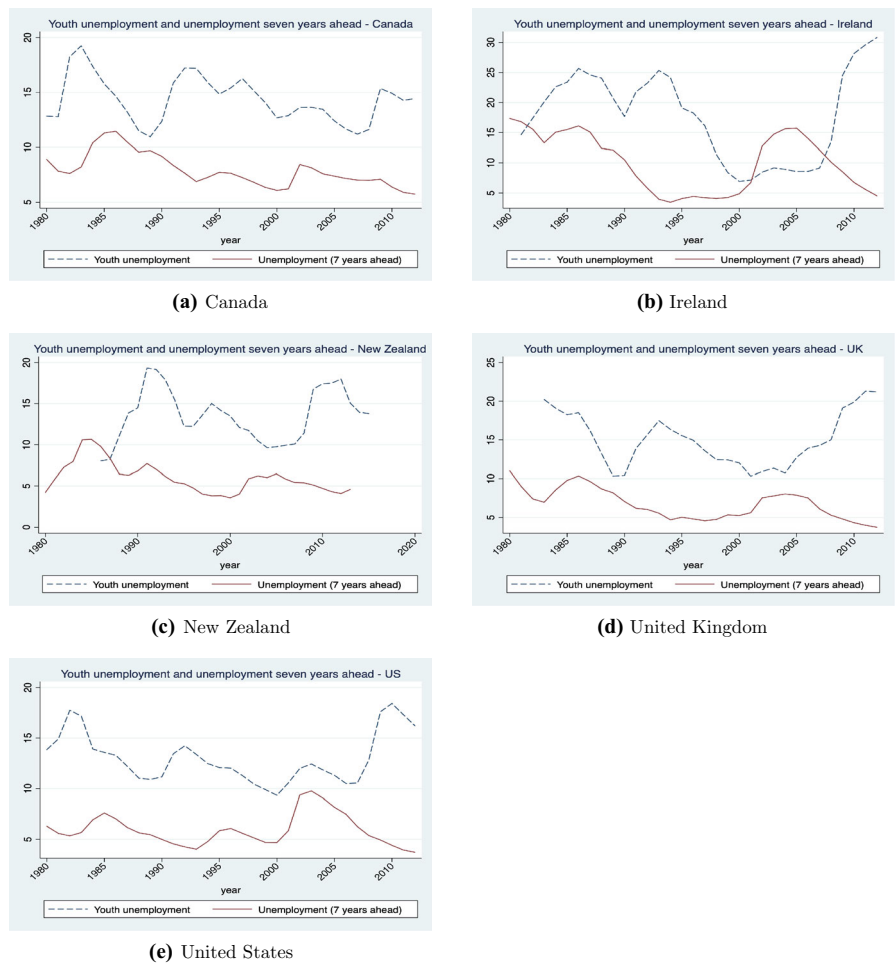
Fig. 3 Youth unemployment and total unemployment seven years later: Anglo-Saxon countries
