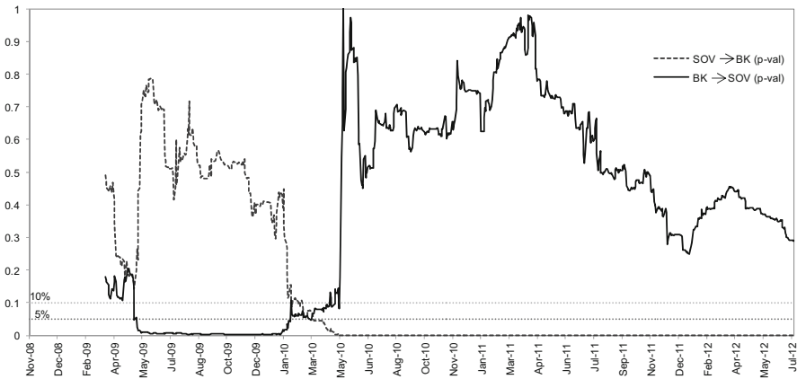
Fig. 3 Recursive Granger-causality tests ( p values)
