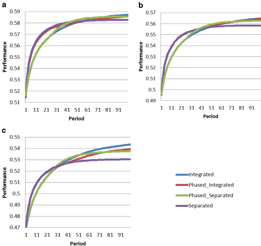
Fig. 4 Performance development with no complementary interdependencies and varying substituting interdependencies. a Performance development with low number of substituting interdependencies ( k=8 , k_s=4 , k_c=0 ). b Performance development with medium number of substituting interdependencies ( k=8 , k_s=6 , k_c=0 ). c Performance development with many substituting interdependencies ( k=8 , k_s=10 , k_c=0 )
