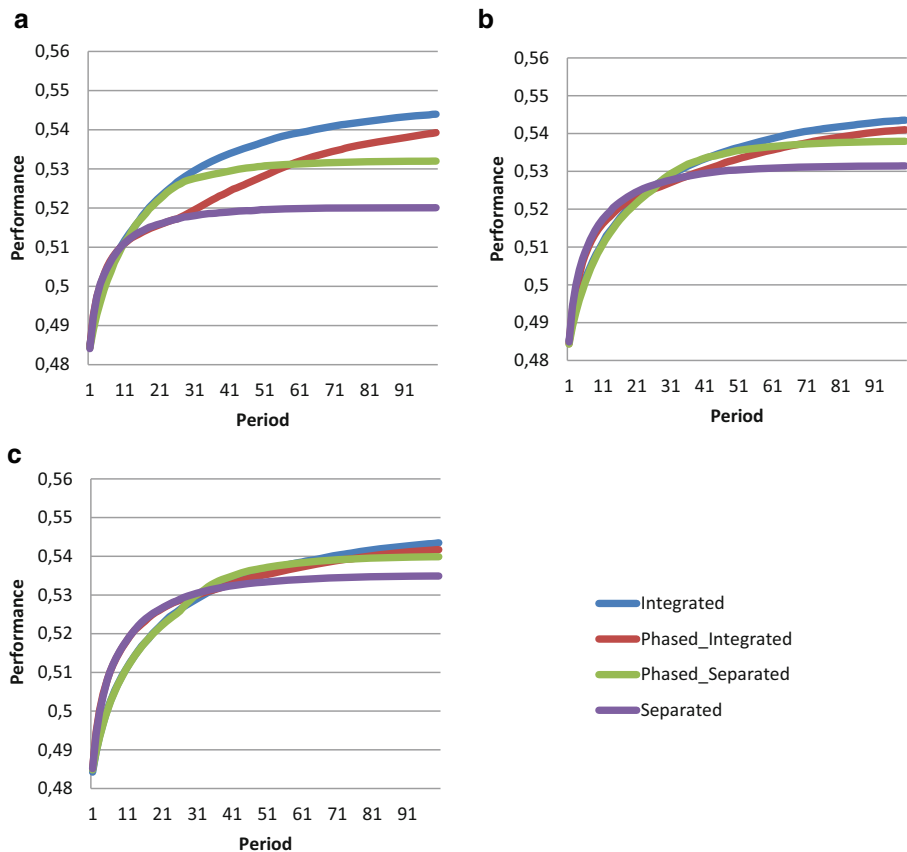
Fig. 6 Performance development with varying degrees of inter-business model visibility. a Performance development with no (0%) inter-business visibility ( k = 8 , k_s = 10 , k_c = 2 ). b Performance development with medium-to-high (75%) inter-business visibility ( k = 8 , k_s = 10 , k_c = 2 ). c Performance development with high (100%) inter-business visibility ( k = 8 , k_s = 10 , k_c = 2 )
