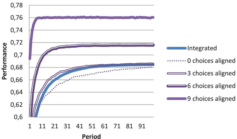
Fig. 8 Performance development—Separated firms with aligned choices ( N=12 , k=4 , k_{\text{inter}}=3 )
