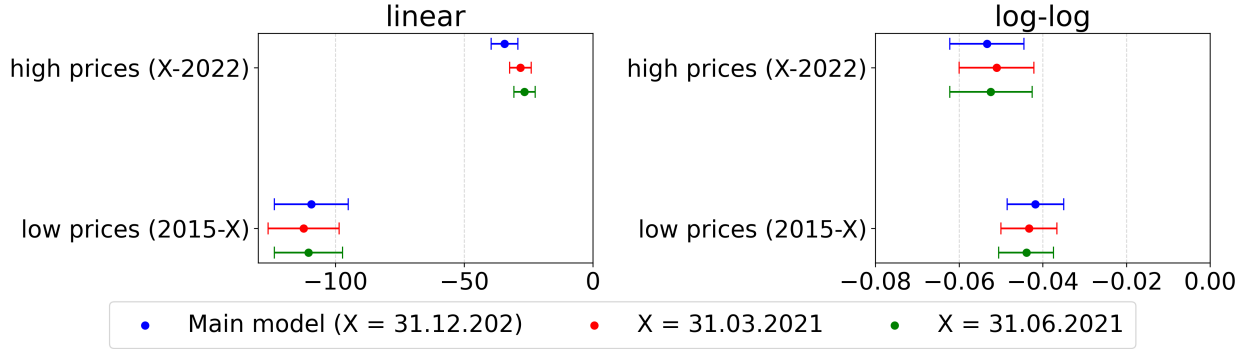
Figure F.19: Estimators for the price effect on demand for the linear (left) and log-log model specification (right), separately for low and high price time subsets. Results are shown for the main model specification (Table 3 and Table 4) (blue) and two model specifications with differing separation dates (X) between the low price time period and high price time period. Whiskers indicate the 95% confidence interval.
