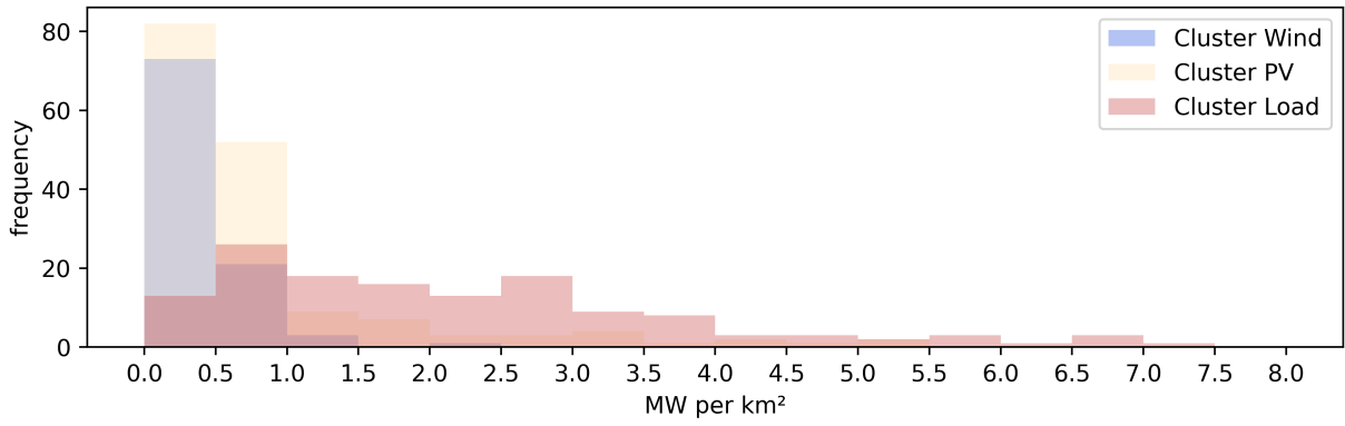
Figure G.8: Distribution of rooftop PV capacities per km^2 within each cluster in 2045
