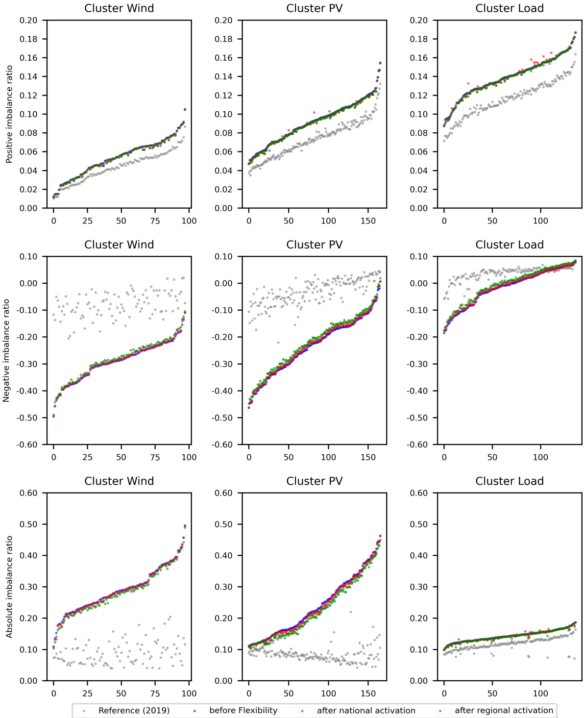
Figure 11: Imbalance ratios before and after the use of flexibility in 2030
