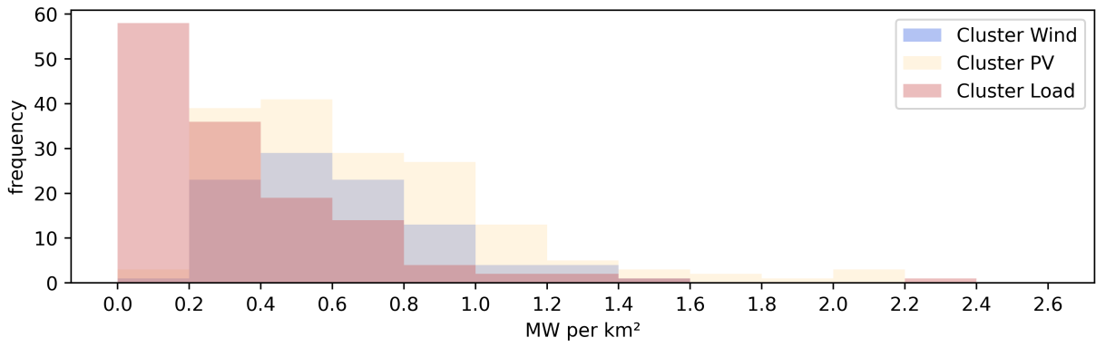
Figure G.7: Distribution of large-scale PV capacities per km^2 within each cluster in 2045
