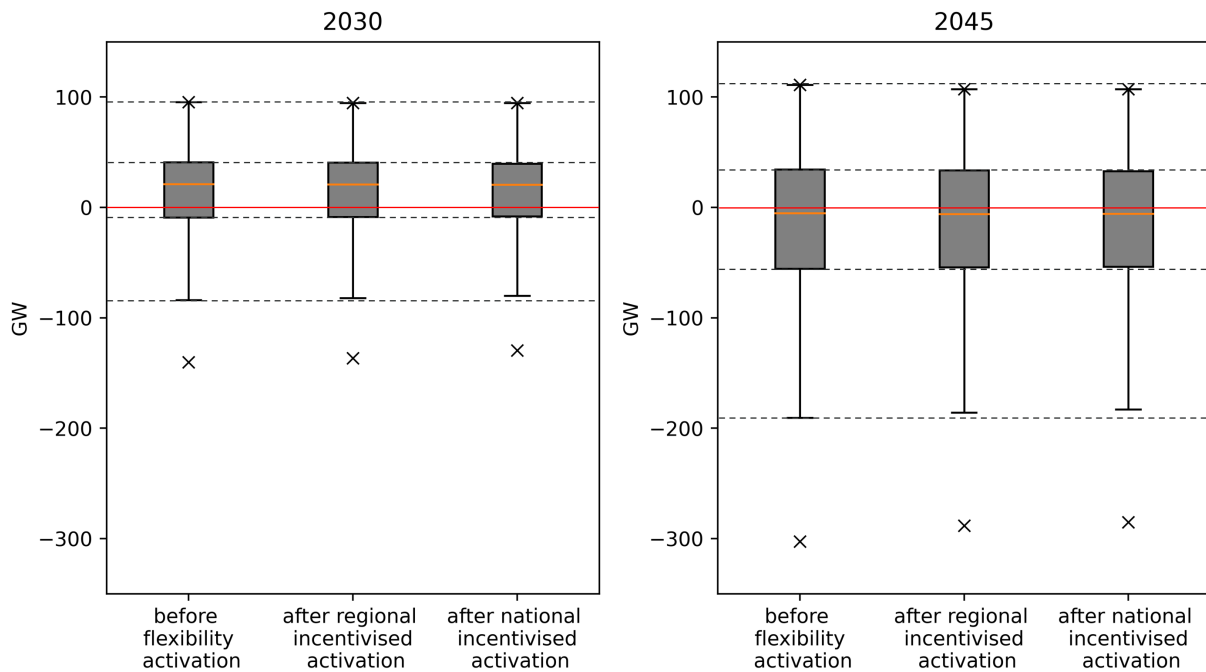
Figure 10: Properties of the national residual load curve before and after the use of flexibility
