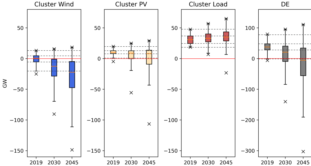
Figure 8: Comparison of regional residual load curves prior to the activation of flexibility
