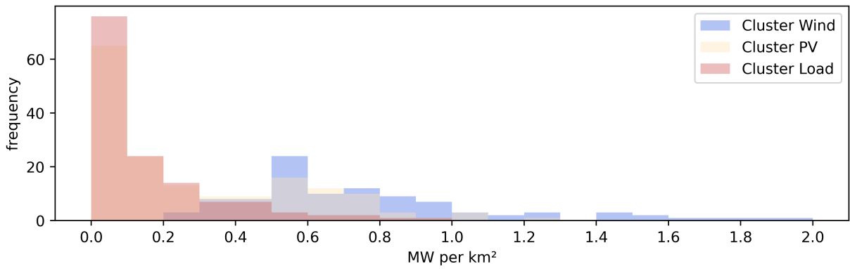
Figure G.5: Distribution of Wind Onshore capacities per km^2 within each cluster in 2045
