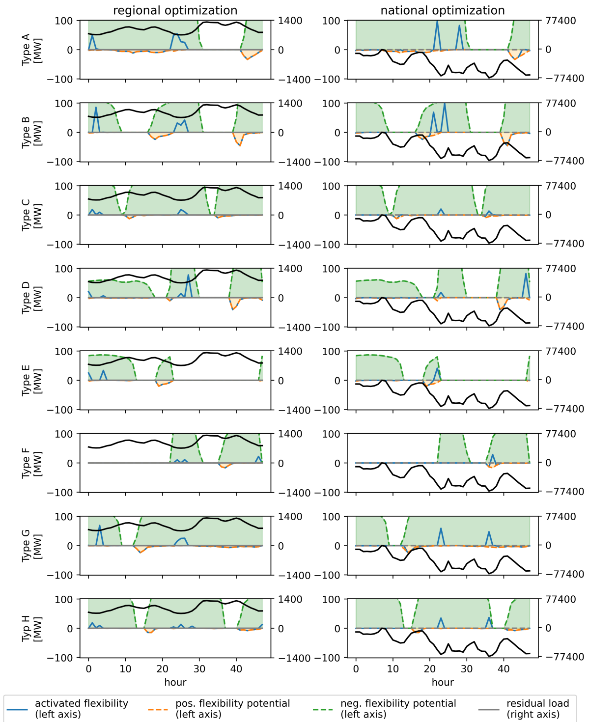
Figure 9: Optimal activation of flexibility in region DE111 (Stuttgart)
