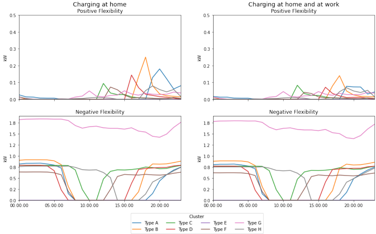
Figure 6: Selected flexibility profiles for a medium-sized city in 2045
