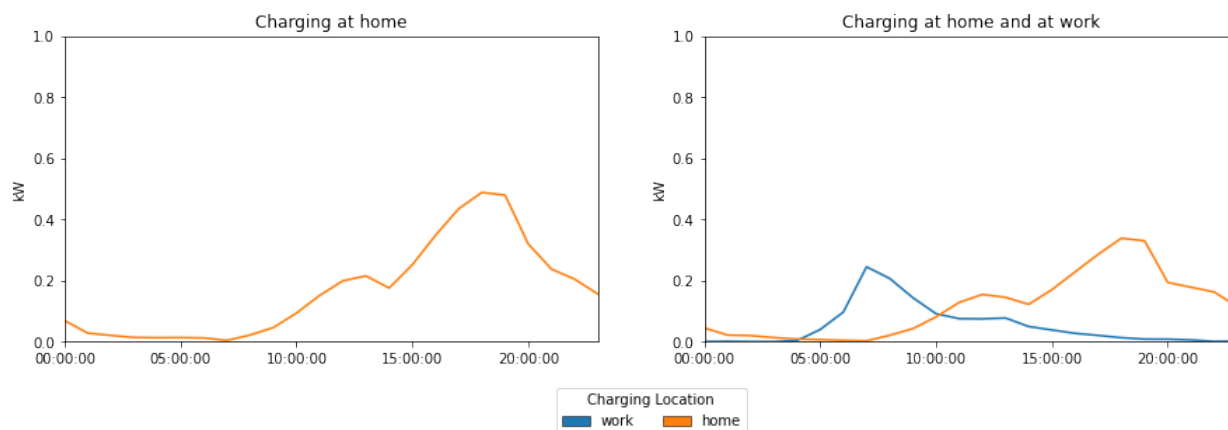
Figure 3: Selected load profiles for a medium-sized city in 2045
