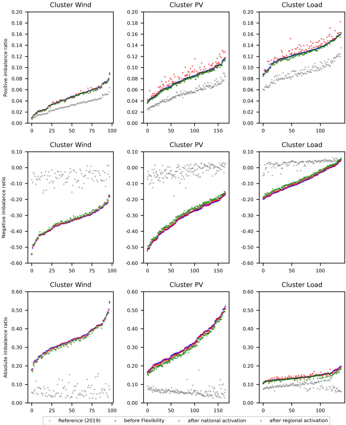
Figure 12: Imbalance ratios before and after the use of flexibility in 2045
