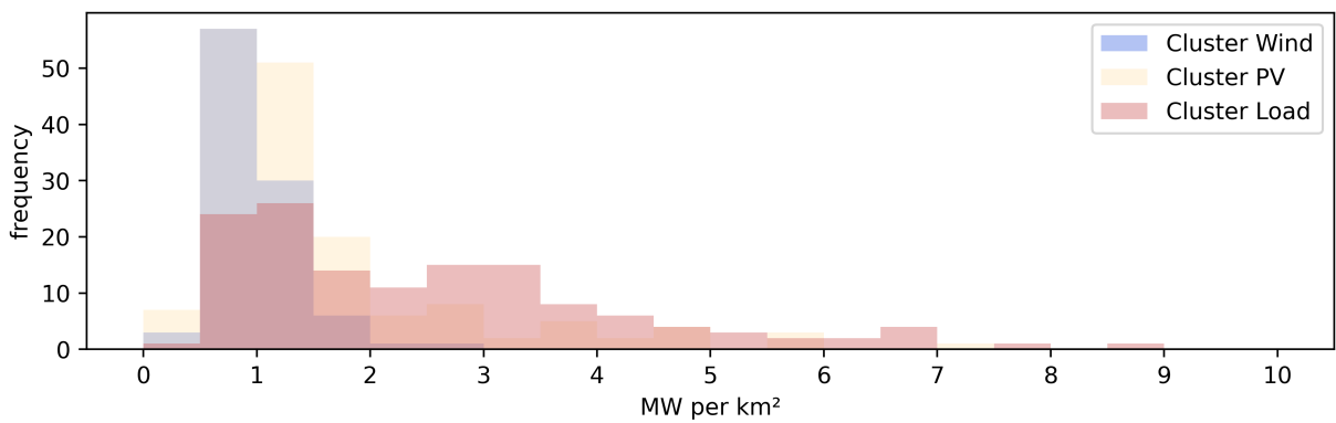
Figure G.6: Distribution of PV capacities (large-scale PV and rooftop PV) per km^2 within each cluster in 2045
