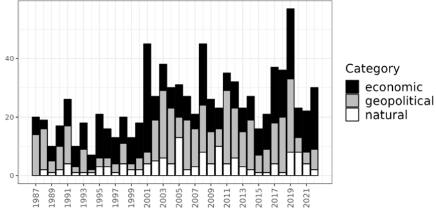
Figure 1: Event distribution
