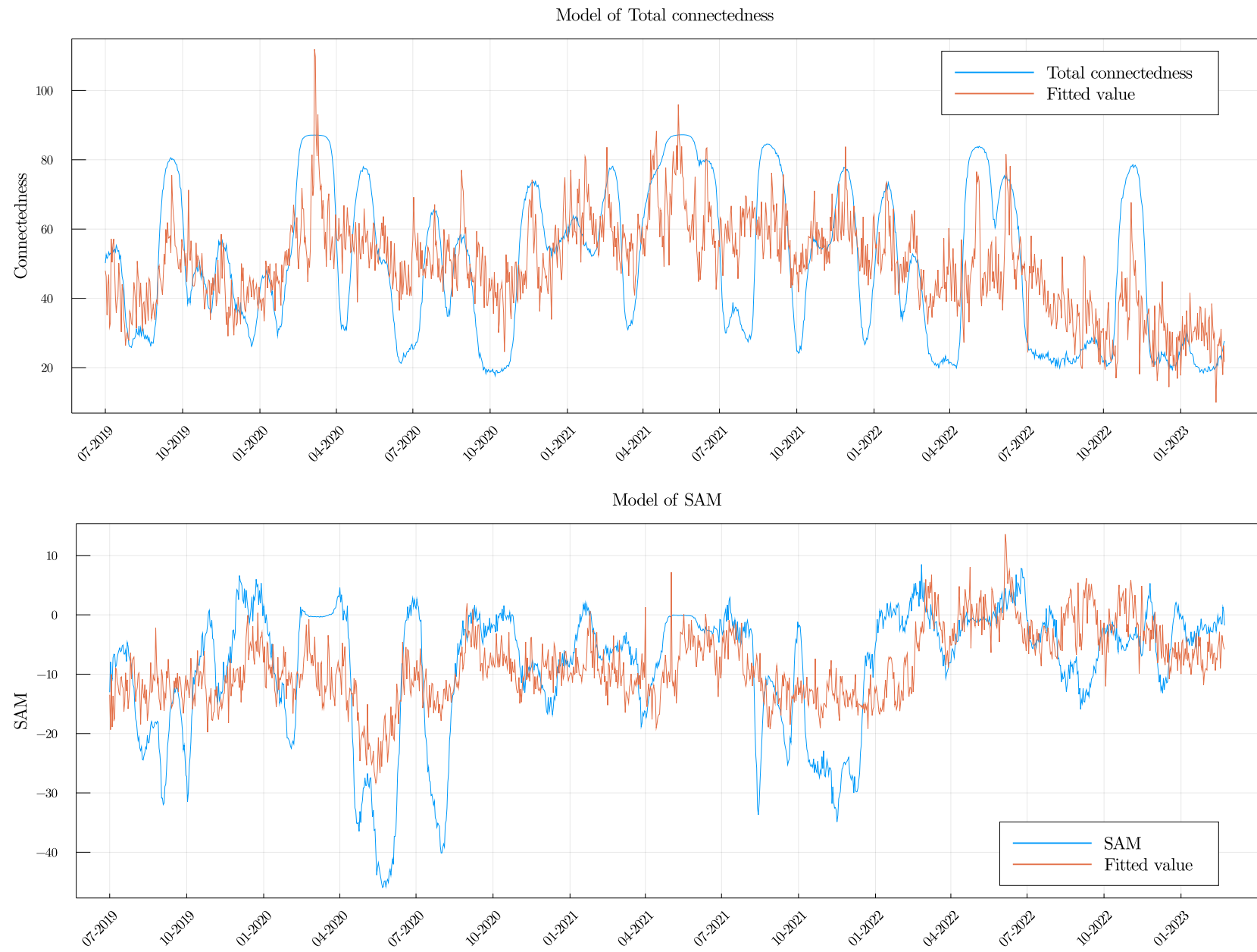
Figure 4: Models of total connectedness and SAM .
