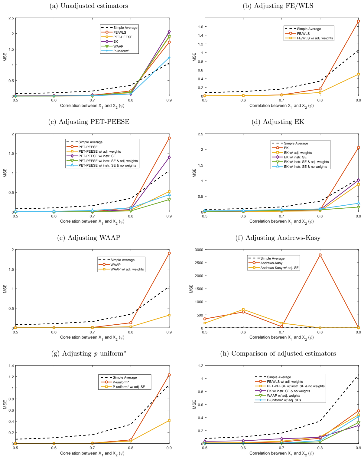
Figure 16: MSE: p -hacking selection, positive effect ( \alpha_1 = 1 ), various values of \psi
