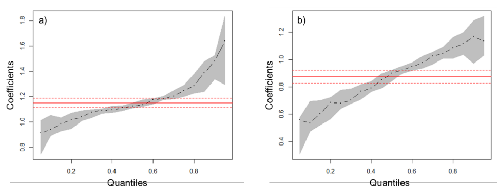
Figure 2.4: Estimated results of quantile regressions for monthly scale precipitation by (a) GSMaP and (b) CHIRPS in Djizzakh station
