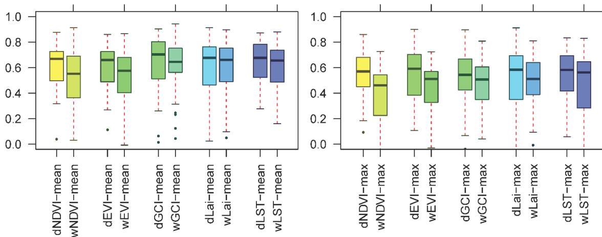
Figure A.2.3.2: Boxplot of correlation coefficients between rainfed wheat yields in Mongolia and mean/max values of indices for the entire district area, croplands and wheatlands; Note: Statistical significance of Wilcoxon test is indicated by following p-values: *p \leq 0.05 , **p \leq 0.01 , ***p \leq 0.001
