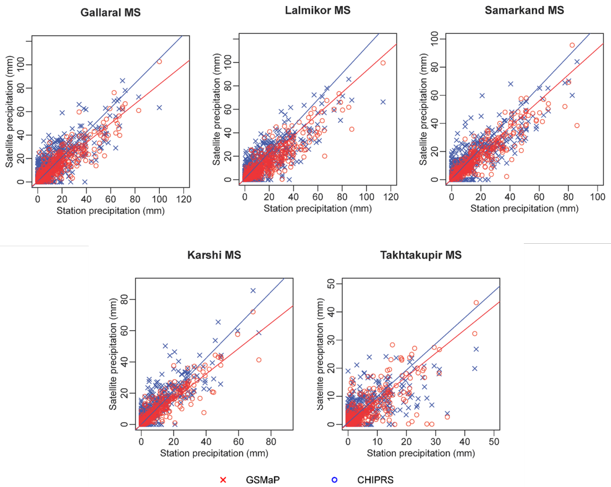
Figure A.1.7.2: Decadal precipitation by stations vs GSMaP and CHIRPS in selected locations
