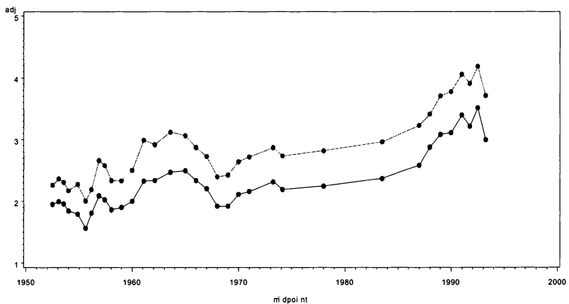
Figure 4: Distrubution-neutral growth elasticities, \eta_1 (top) and \eta_2 (bottom), absolute values*
