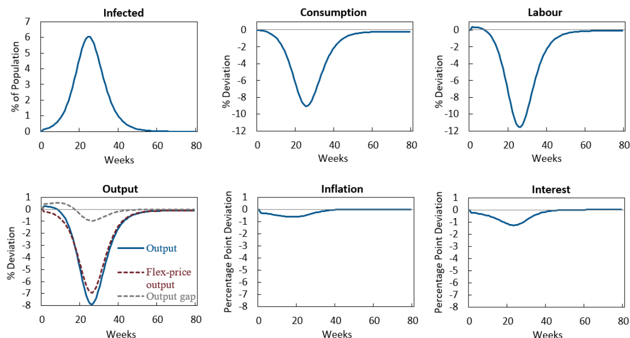
Figure 7 Simulation of an epidemic in a New-Keynesian macro-epi model
