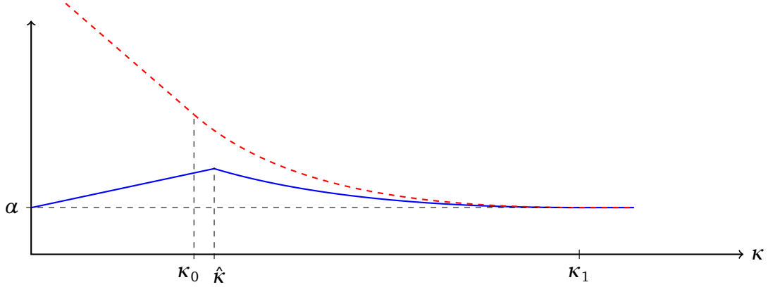
Figure 2: Total equilibrium welfare (blue) and first-best welfare (red, dashed) for the cost specification (49) as a function of \kappa for the values \alpha = 1 , \omega = 3/2 , \kappa_0 = 1/12 , \kappa_1 = 1/2 .
