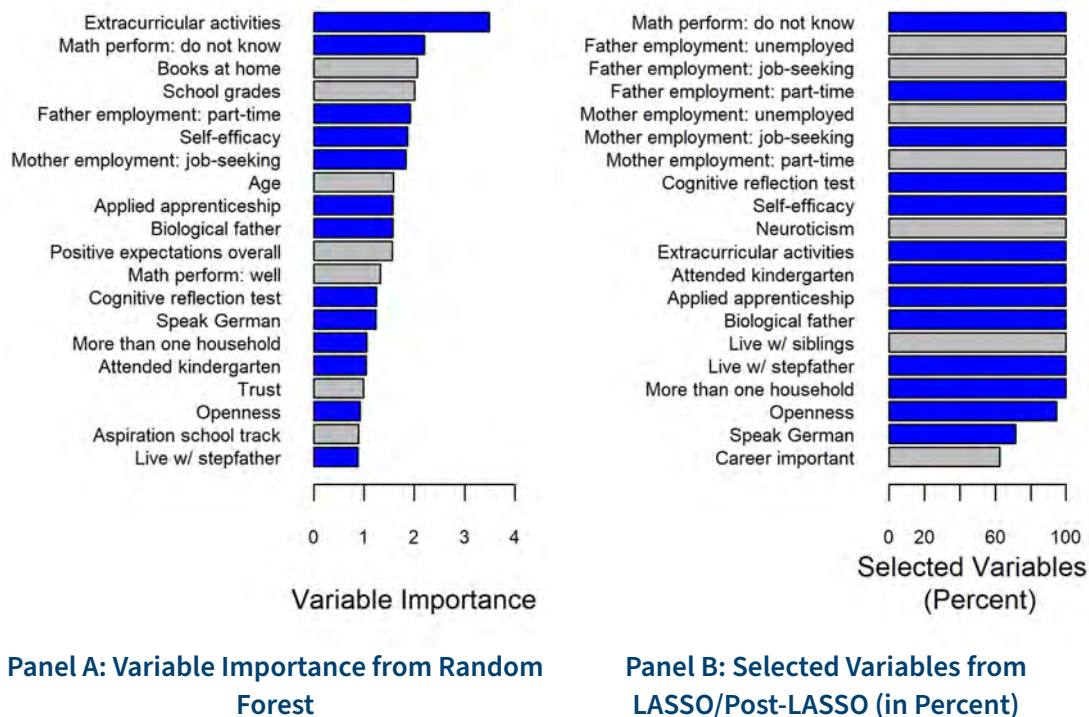
Figure 3.2: Important Predictors
