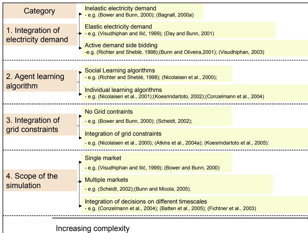
Figure 6: Examples for the increasing complexity of agent-based simulations
