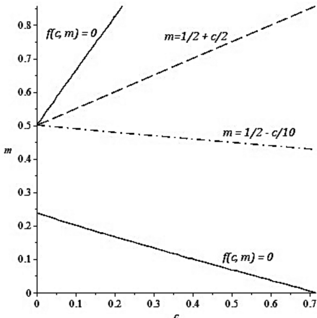
A PLOT OF f(c, m) = 0 WHEN m \geq \frac{1}{2} - \frac{c}{10} IN REGIME B
