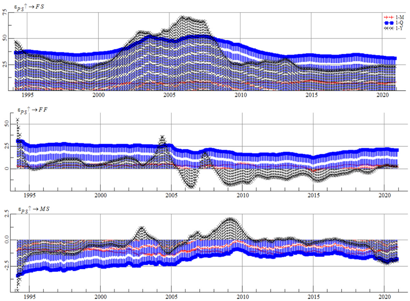
FIGURE 1 TVP-VAR MODEL: TIME-VARYING RESPONSE TO SHOCKS IN THE PRICE STABILITY
