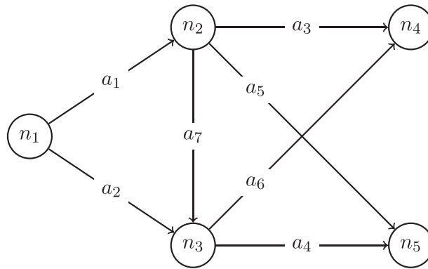
Fig. 1. 5-node network.
