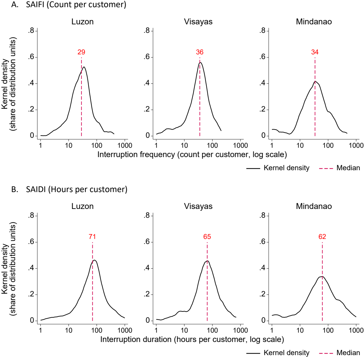
Figure 2. Distribution of electricity system interruption indices by broad region, 2010-2022
