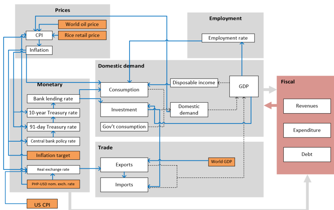
Figure 1. The PIDS small macroeconometric model
