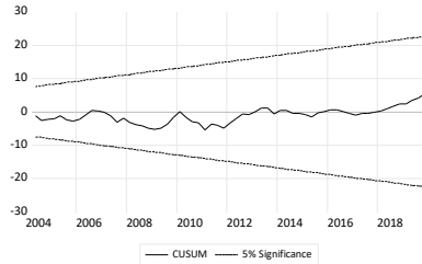
CUSUM test
