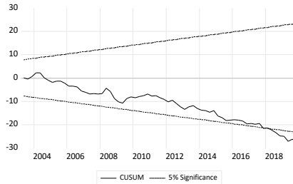
CUSUM test
