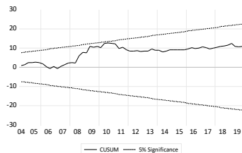
CUSUM test
