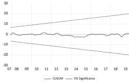
CUSUM test
