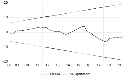
CUSUM test
