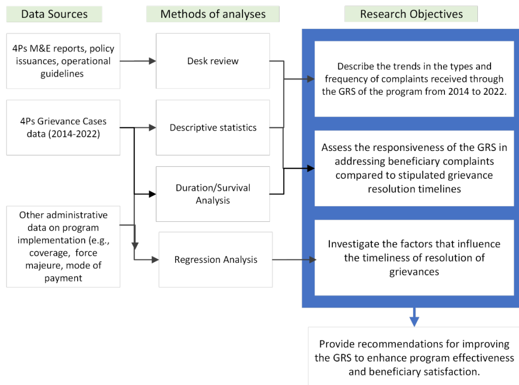
Figure 4. Methodological framework
