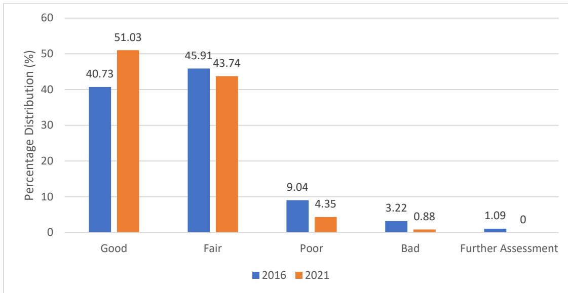
Figure 6. Condition of national bridges, 2016 vs. 2021
