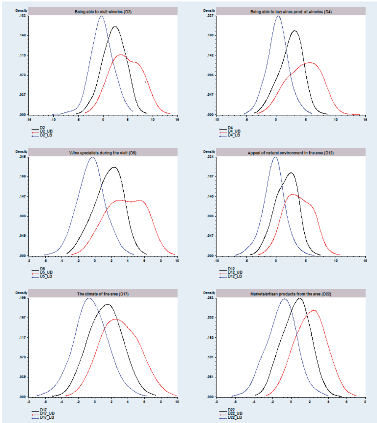
Figure 2. Distribution of random coefficients. Kernel density estimates.
