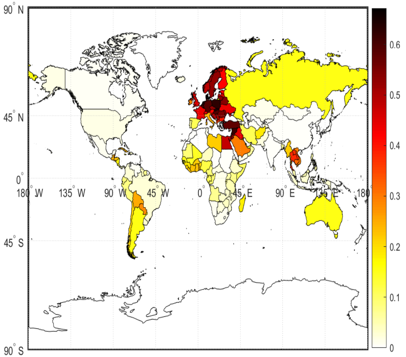
Figure A.1: Contribution of the regional factor to temperature volatility
