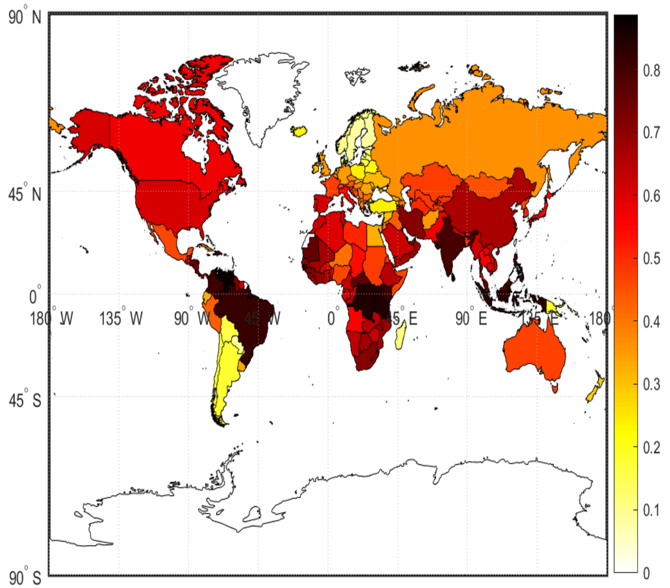
Figure 4: Contribution of the world factor to temperature volatility. Average across time
