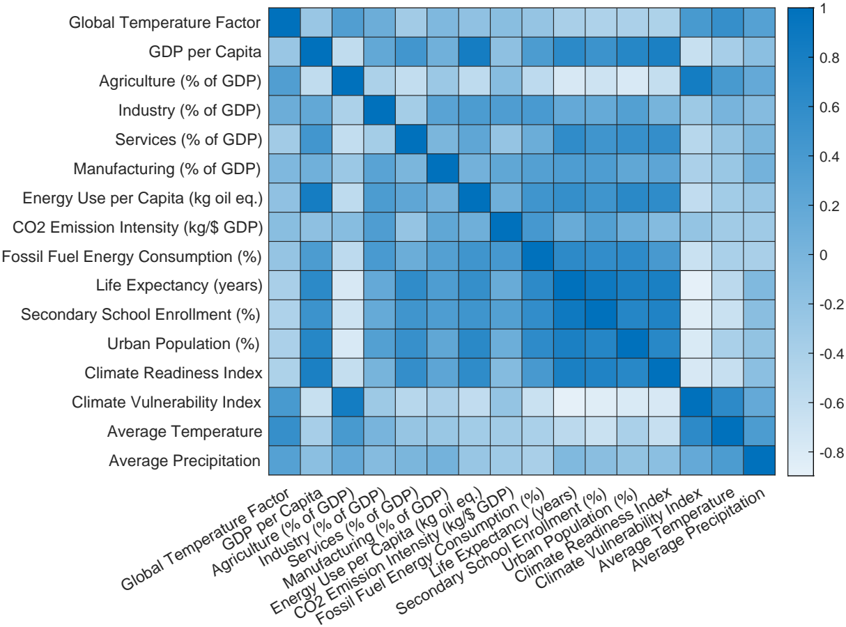
Figure 6: Vulnerability and country characteristics: correlation heatmap
