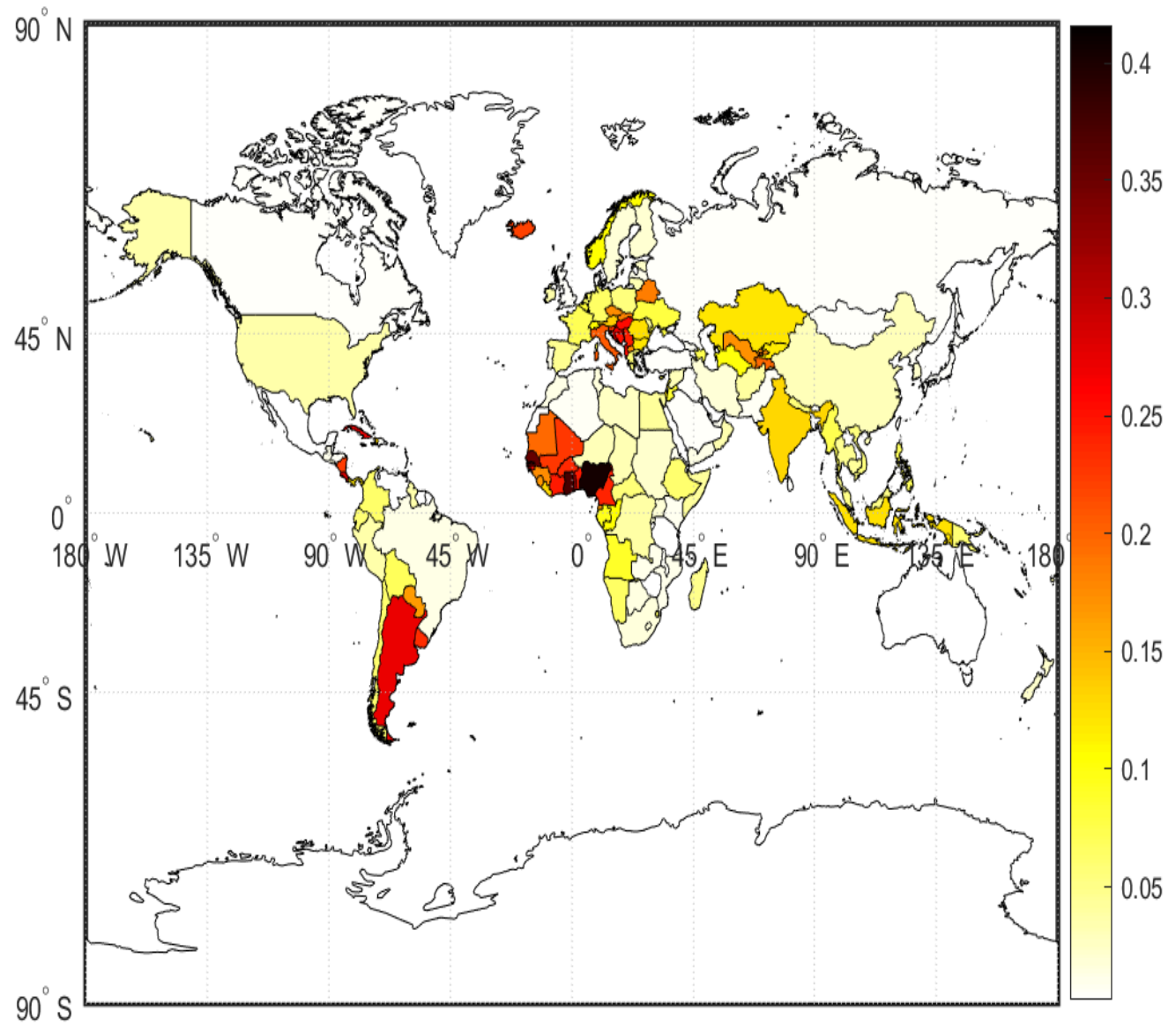
Figure 5: Contribution of the world factor to precipitation volatility. Average across time.
