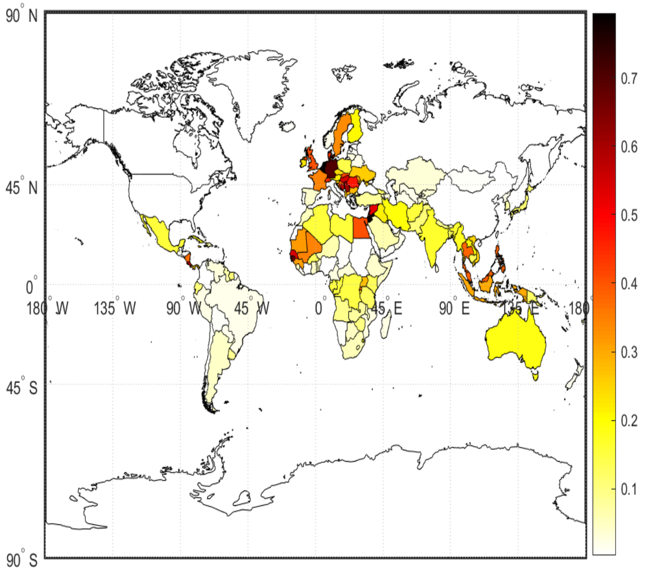
Figure A.2: Contribution of the regional factor to precipitation volatility
