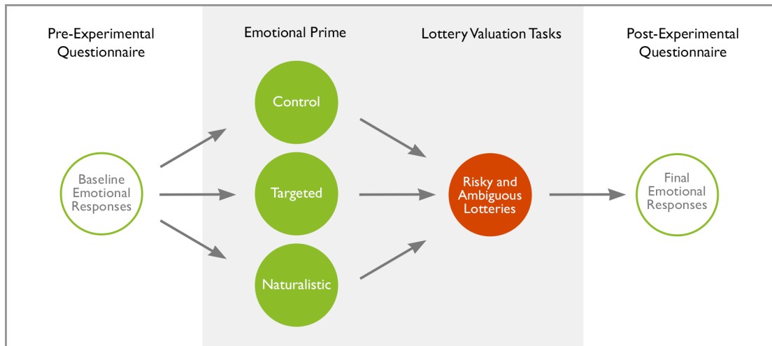
Fig. 1 Experimental design
