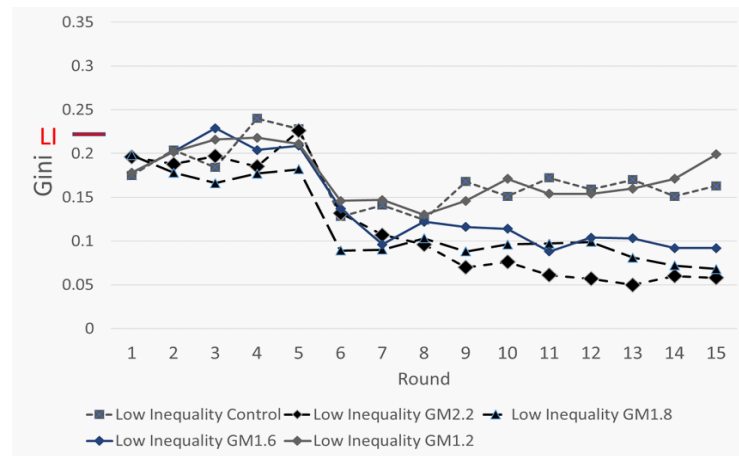
Figure 2: Gini Coefficients
