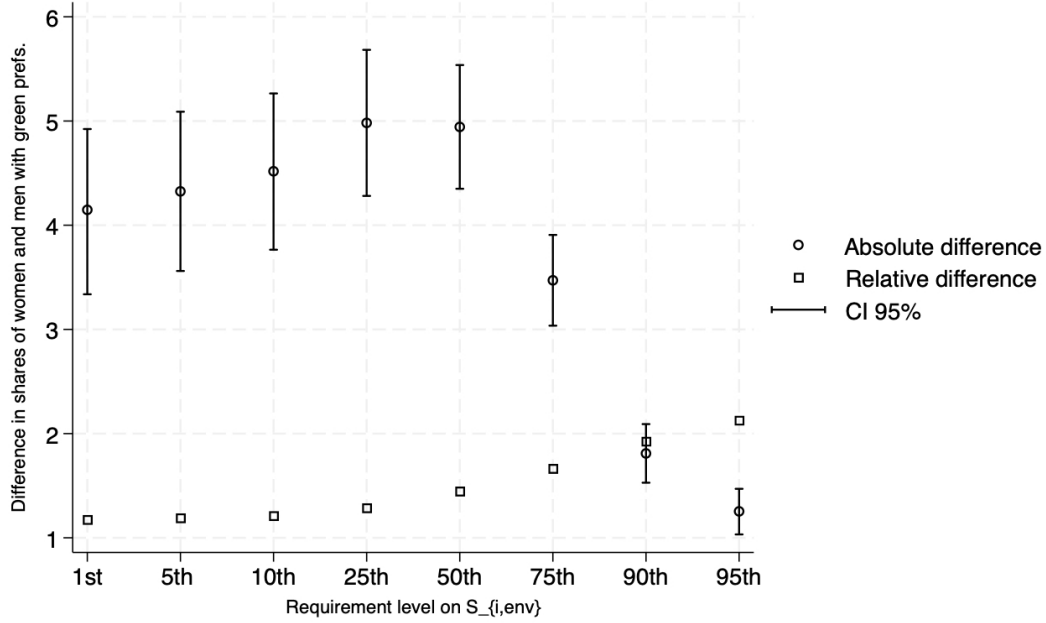
Figure 5: Extensive margin.
