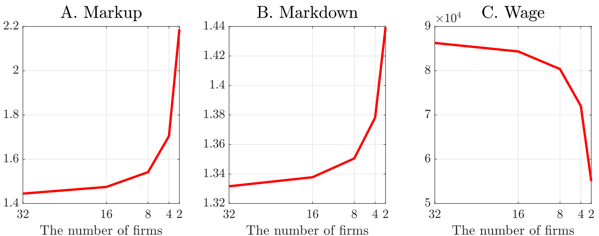
Figure 1: Comparative Statics
