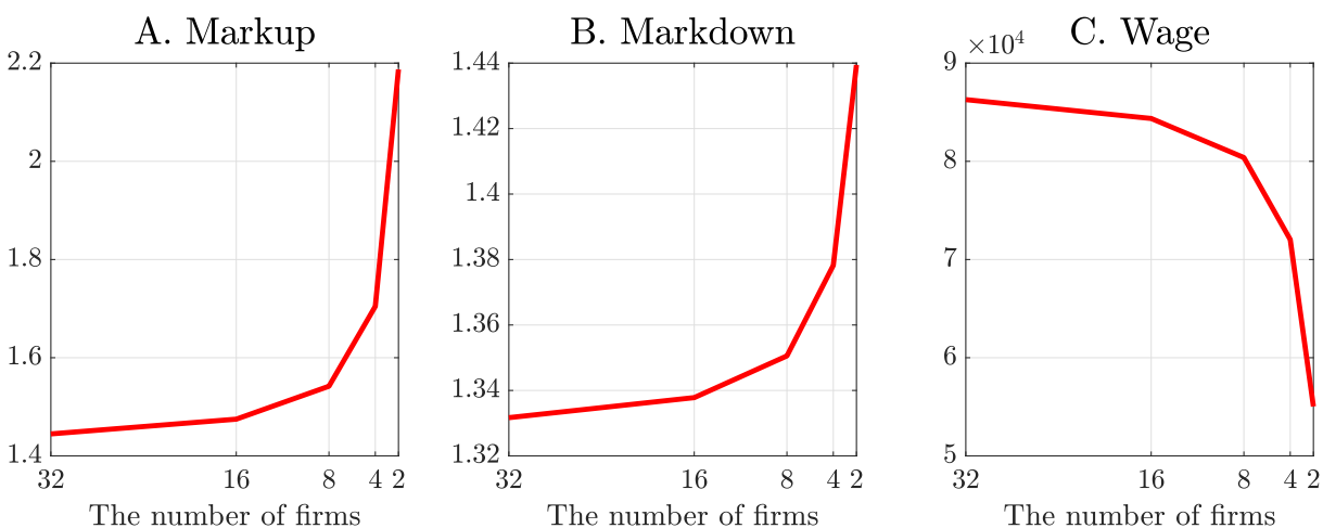
Figure 1: Comparative Statics
