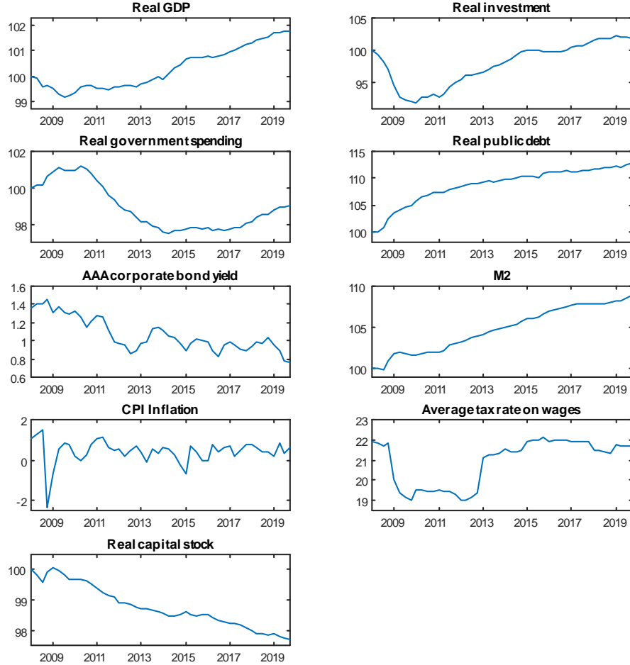
Figure 4: The data
