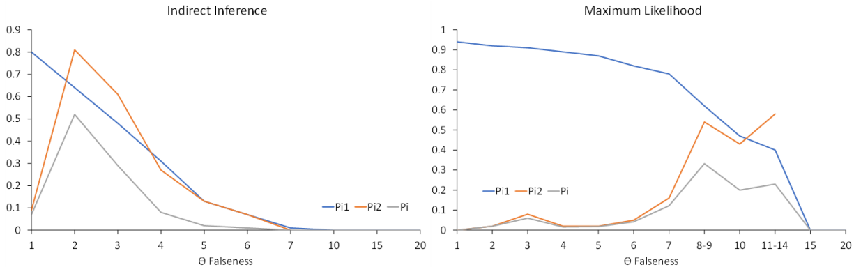
Figure 3: Predicted probabilities and biases for II and ML
