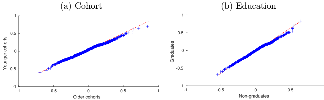
Figure A25: Quantile-quantile plots for \xi_i by observables
