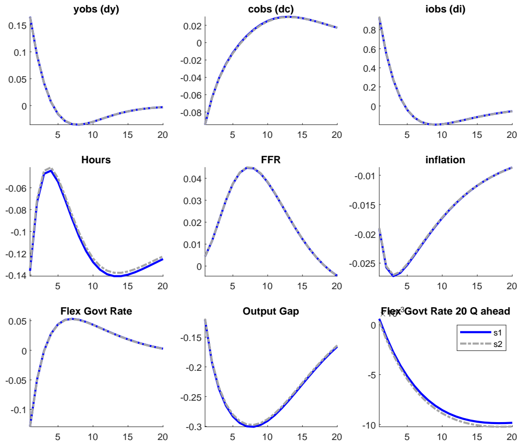
Figure 5: InvestmentShock
