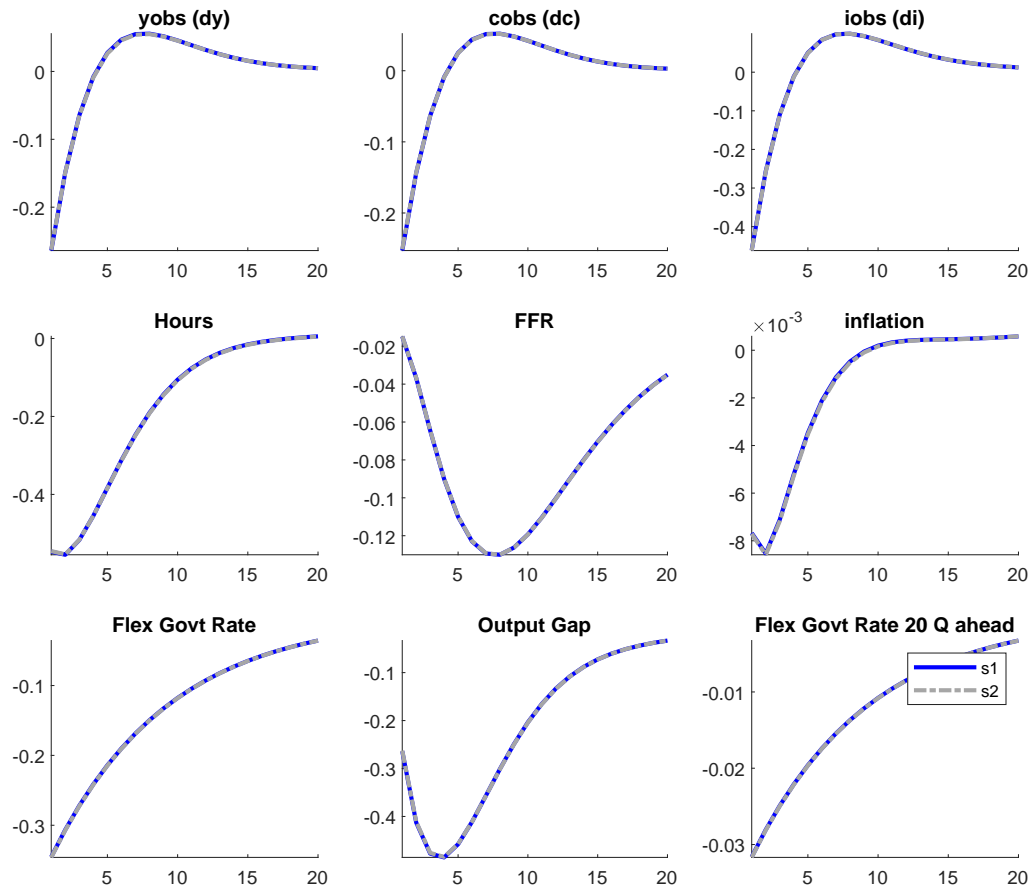
Figure 9: LiquidityPreference
