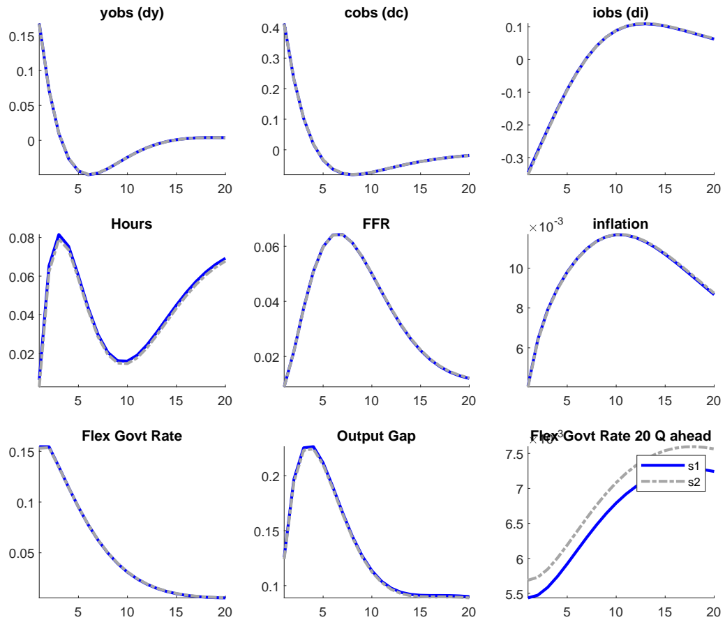
Figure 1: DiscountFactor
