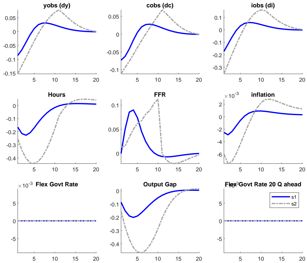
Figure 4: FactorB
