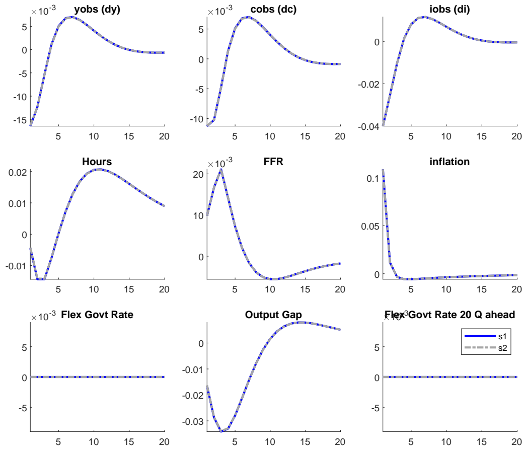
Figure 7: PriceMarkup
