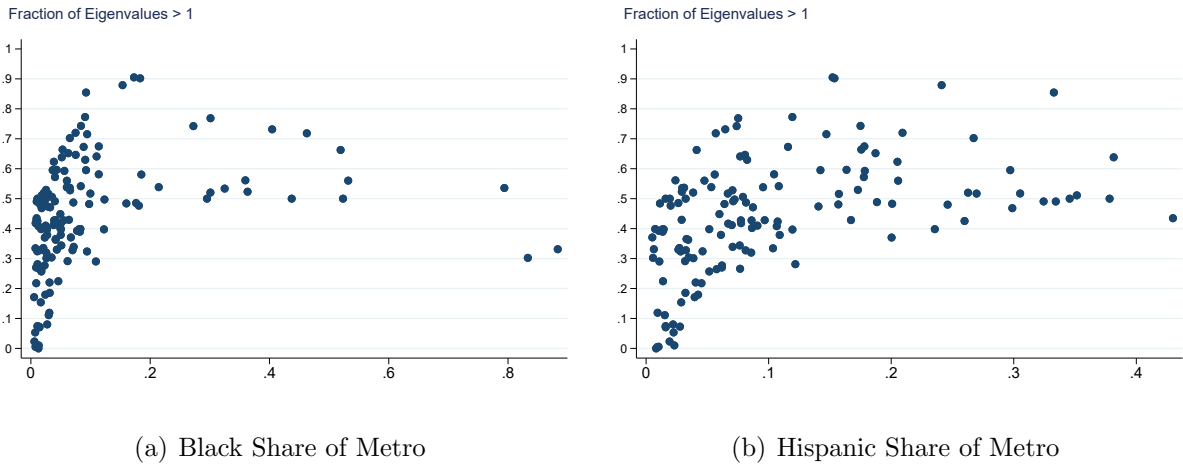
Figure 5: Fraction of Metro Eigenvalues > 1
