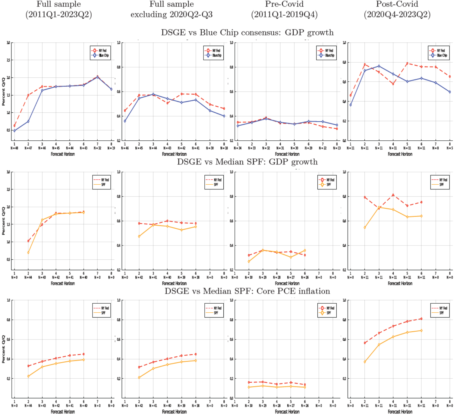
Figure 1: Out-of-sample RMSEs
