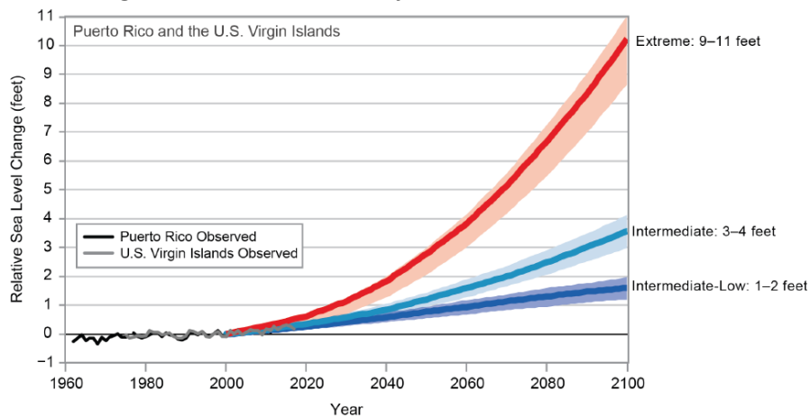
Figure 5. Observed and Projected Sea Level Rise
