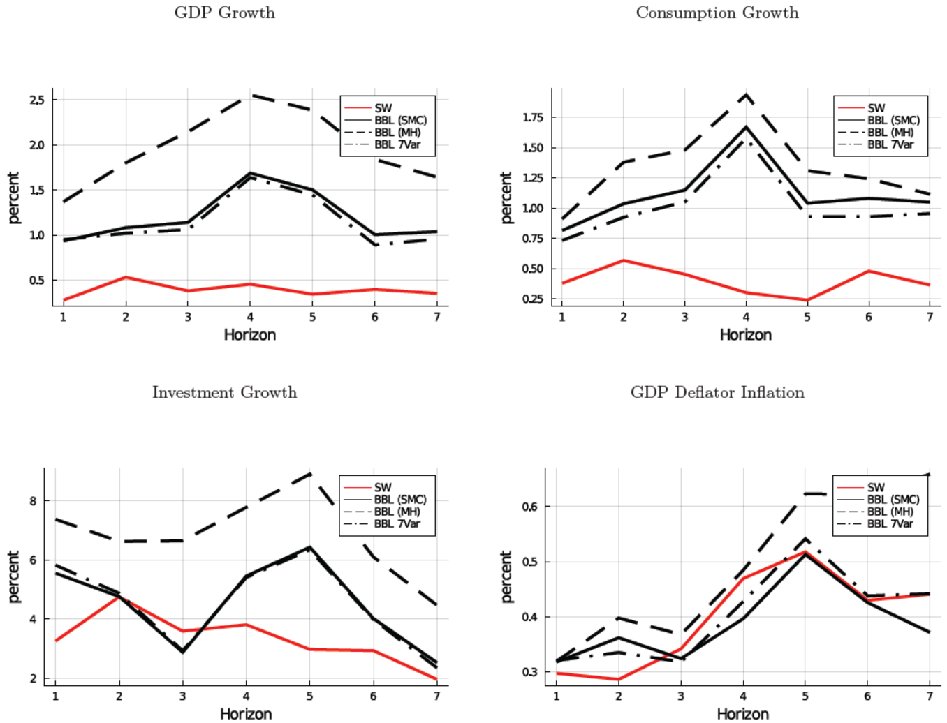
Figure 2: RMSEs: Robustness
