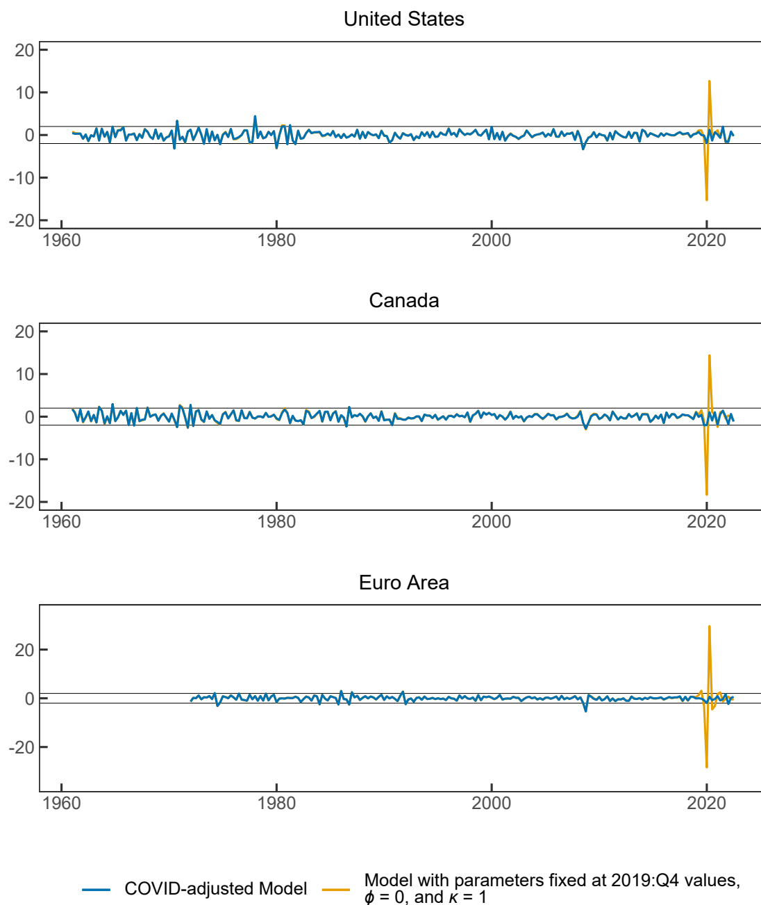
Figure 4: Standardized Auxiliary Residuals: Natural Rate of Output
