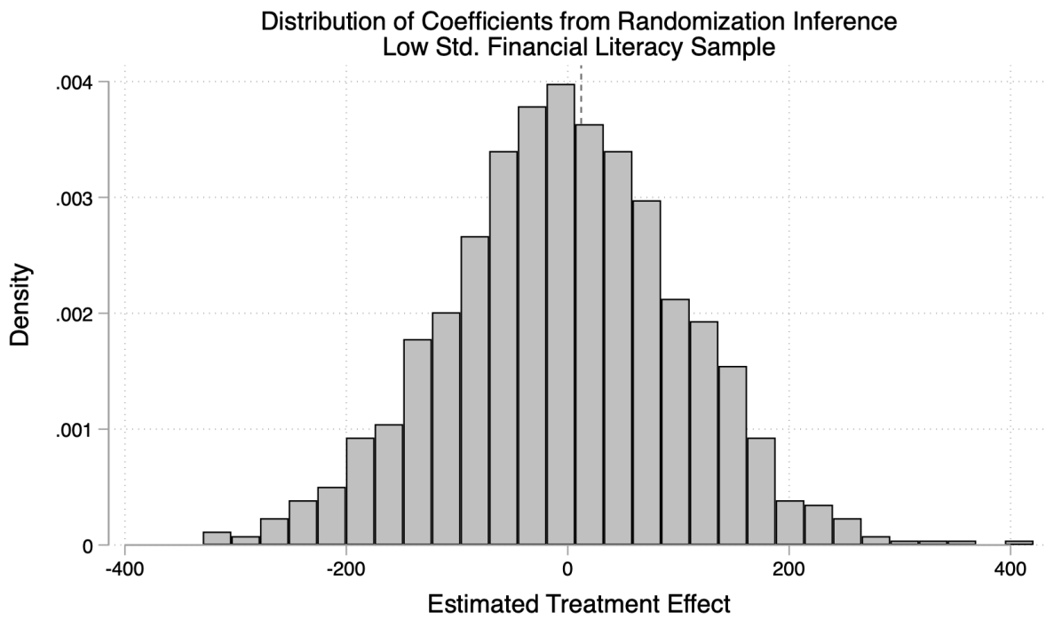
Figure B.6: Randomization Inference Histogram of TOT effect on TSP Amount for Low Financial Literacy Sample
