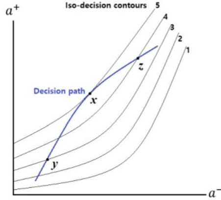
[Figure 2.5: Iso-decision contours and decision path]
