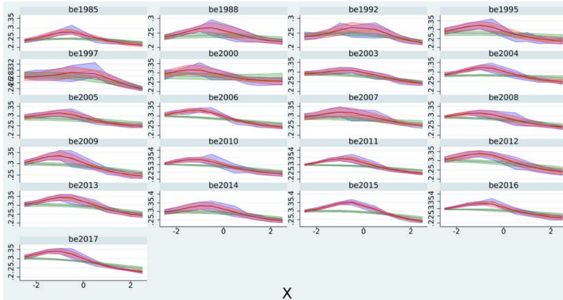
Figure 12: isograph for Belgium 1985-2017 with empirical, gb2, and LaSiPiKa distributions
