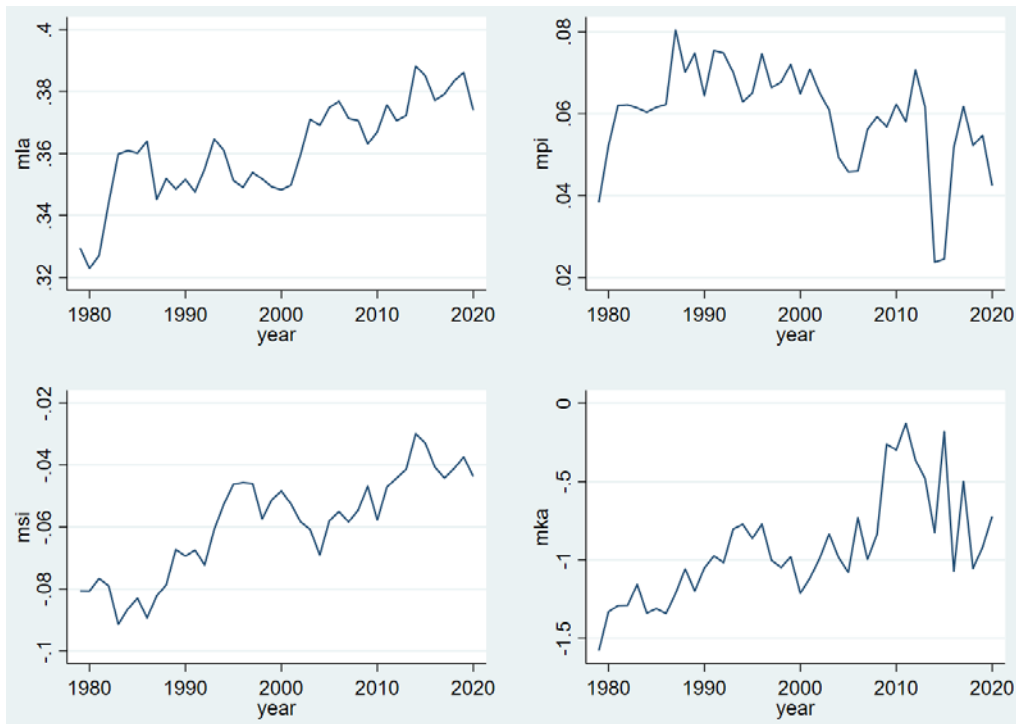
Figure 19: U.S. 1979-2020 gb2(aa, bb, pp, qq) parameters
