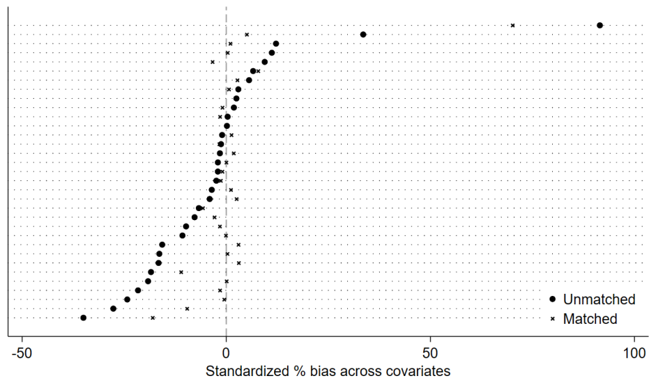
Figure A1: Bias reduction using propensity matching with nearest neighbour
