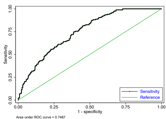
Figure A3: ROC curves for predicting reforms episodes
