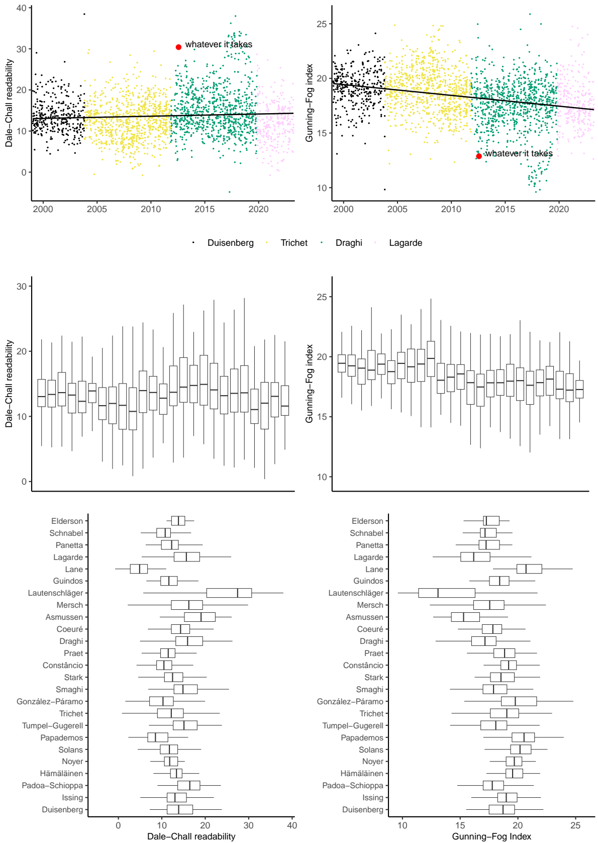
Figure A.3: Dale-Chall score and Gunning-Fog index
